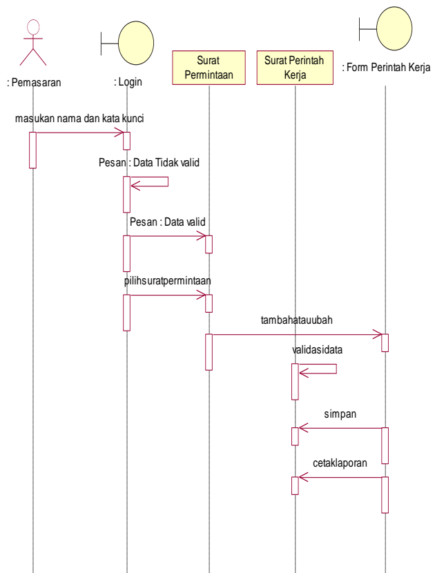
Sumber: Hasil Olahan Data Gambar 6 Sequence Diagram Surat perintah Kerja
