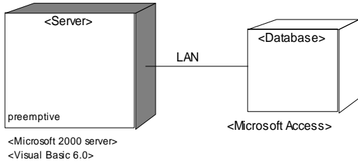
Sumber: Hasil Olahan Data Gambar 13 Deployment Diagram
